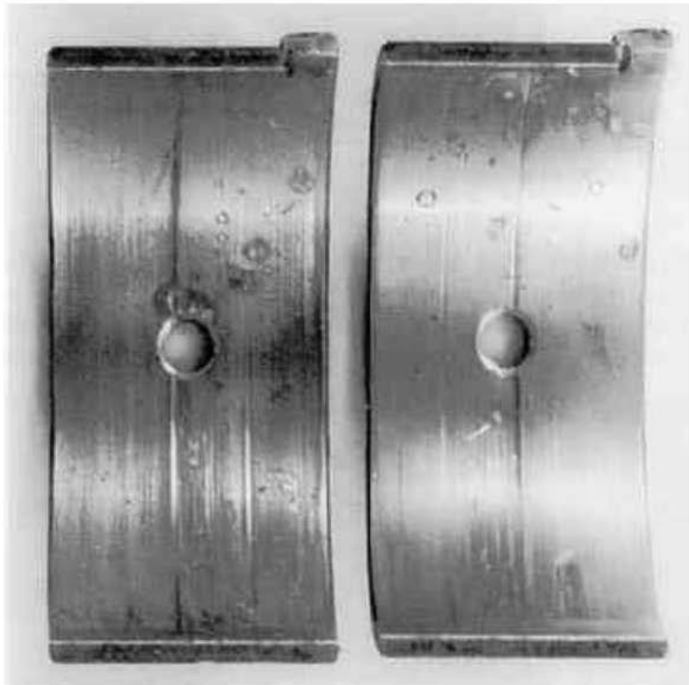
Figure 29 — Embedding of particles, characteristic of embedding, see Figure 28, and migration tracks (material: steel/AlSn)
