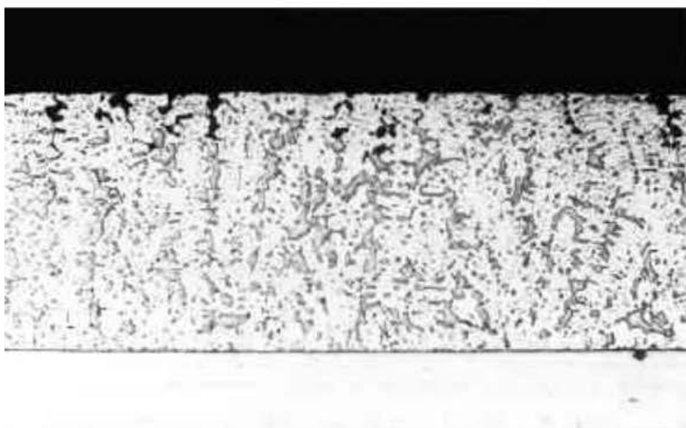
b) microcut at increased magnification (material: steel/lead bronze/electroplated overlay)
